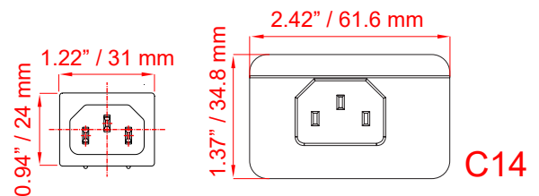
INPUT 100 ~ 240 VAC (IEC320 C14 AC PIN)
