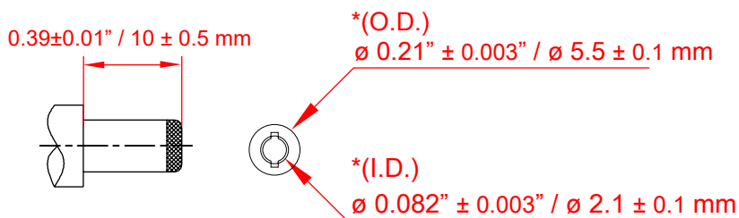
OUTPUT 12V / 5A (DC MATE PLUG)
