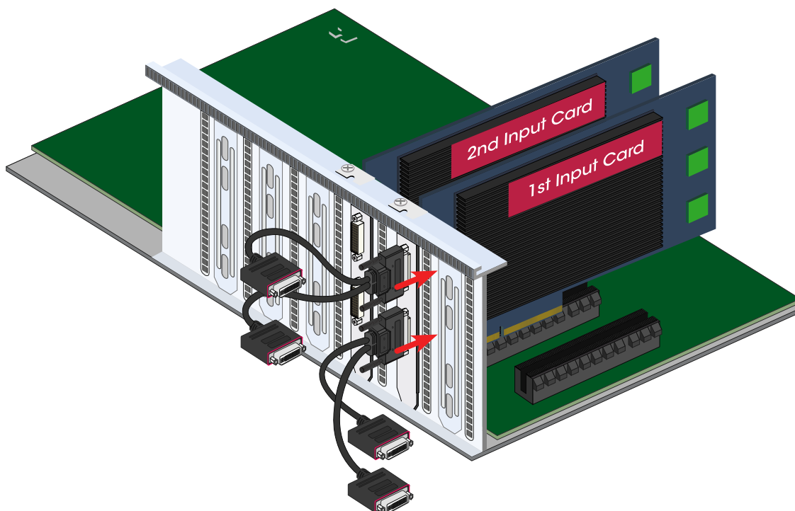
Install cP4 cables
